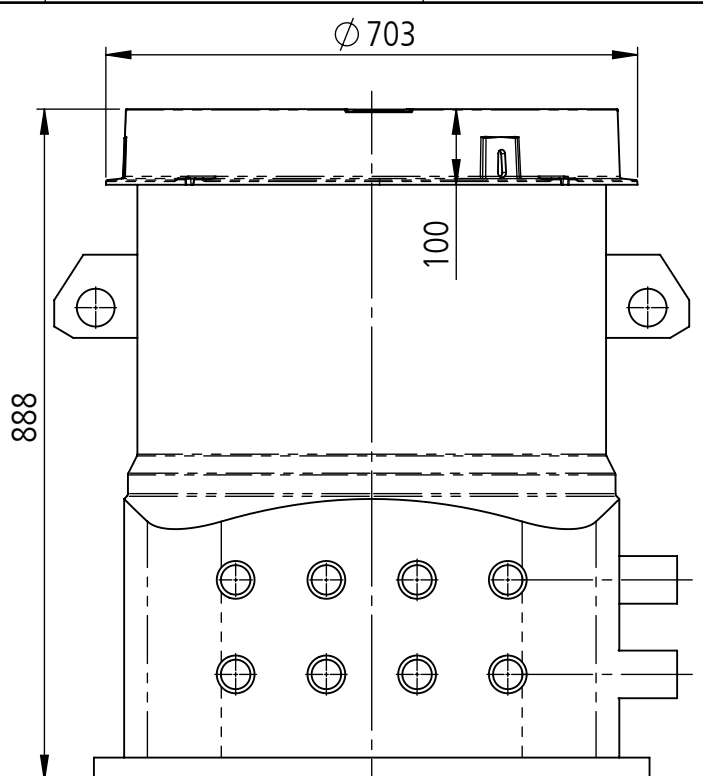
Vollguss Abdeckung B125 verschraubt Couvercle en fonte B125 boulonné Coperchio in ghisa B125 imbullonato Cast iron cover B125 bolted
